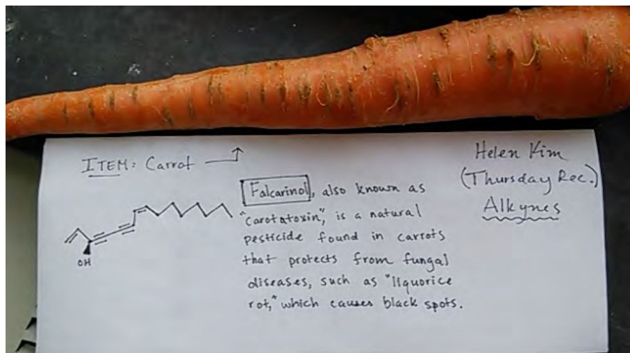
Natural Pesticide: falcarinol
