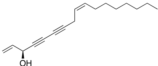
Natural Pesticide: falcarinol
